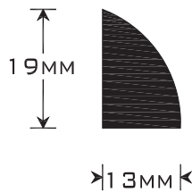
CONVENTIONAL BAMBOO BEAD STRIP
